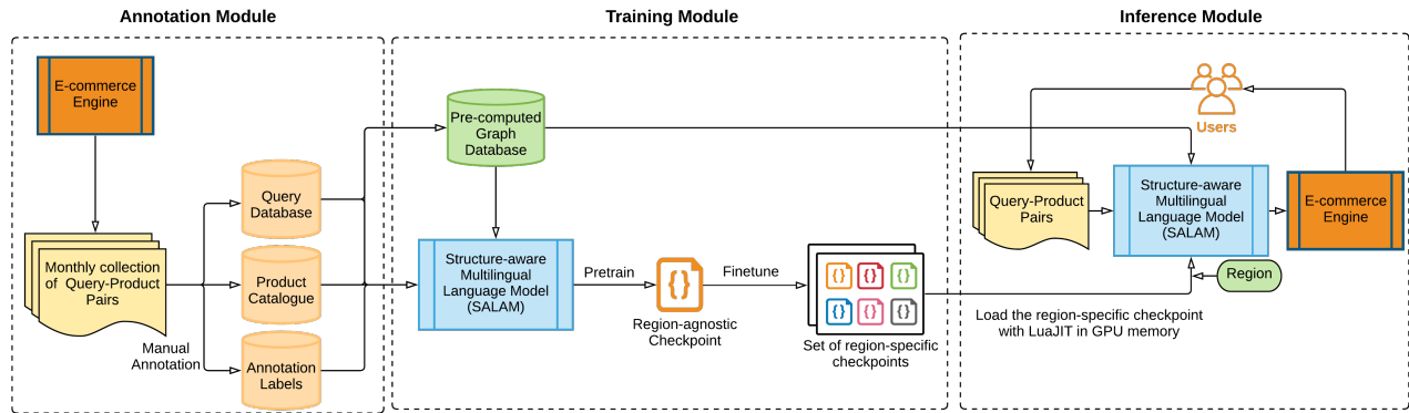
Figure 4: SALAM Workflow. The existing annotation module can seamlessly be integrated with the training and inference module of our model. The additional disk requirement for the pre-computed graph database is trivial and within limits of general industrial settings.
