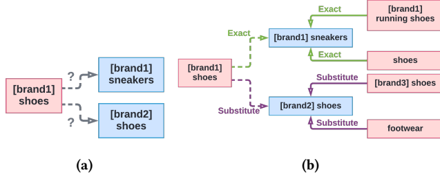
Figure 1: Sample of a query-product pair with (a) only text and (b) text and graph structure. Note that classifying the relation in (a) based only on text is difficult because both the products have a single token match with the query. However, with the aid of graph structure in (b), the classification becomes easier with more semantic token matches and additional information about the relations.
