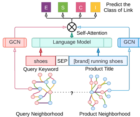
Figure 2: An overview of the proposed SALAM. Given the input query-product pair with their corresponding local neighborhoods, SALAM combines the power of textual and graph representations for ESCI classification.
