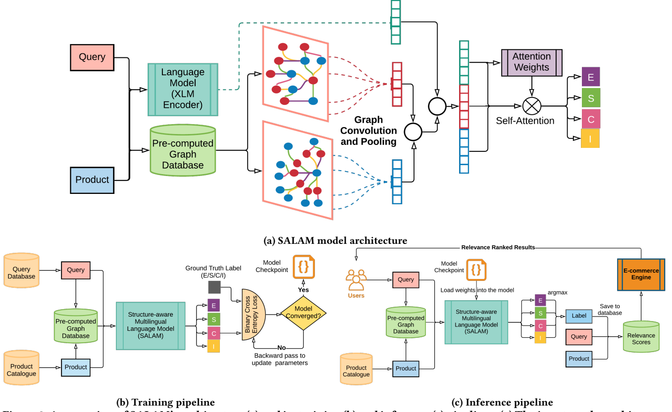
Figure 3: An overview of SALAM’s architecture (a) and its training (b) and inference (c) pipelines. (a) The inputs to the architecture are a query-product text pair with a pre-computed graph neighborhood which is obtained from the purchase information. The textual and graph features are encoded using a language model and GCN, respectively. Subsequently, the concatenation of the features are pooled with an attention mechanism to finally predict the probability of the classes. (b) The training pipeline uses the query database and product catalogue with a ground truth label for back-propagation and saves a model checkpoint on convergence. (c) The inference pipeline employs the checkpoint to classify search relevance on a user query and products from the catalogue to generate the final label, which is stored in the database for relevance computation in the e-commerce engine.
